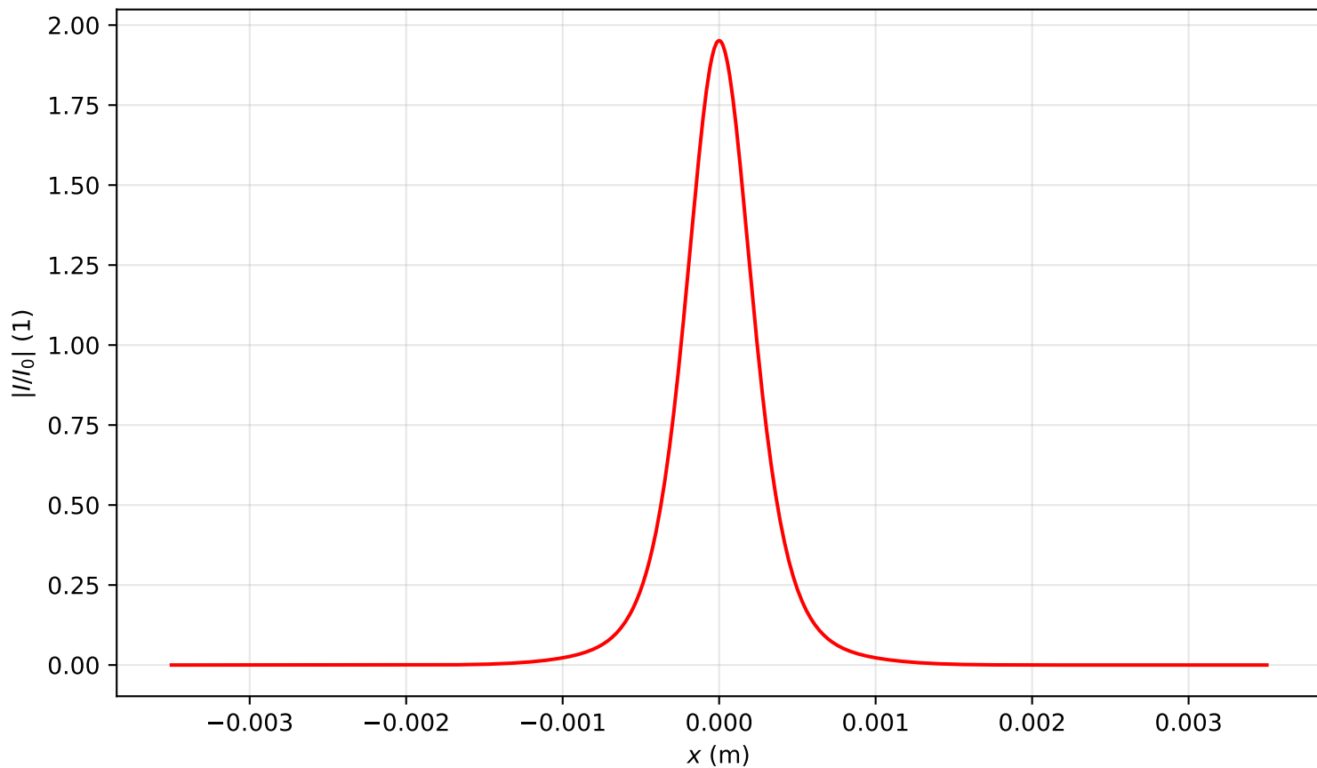
Intensity profile I(x, y = 0, z = 1.672)/I_0 , P_{in}=1.0P_{cr} , artificial time
